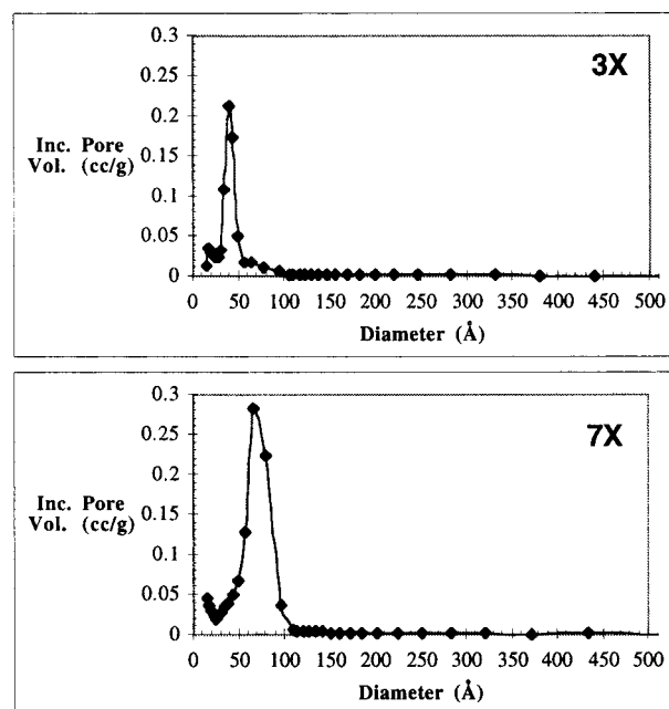
Figure 12. Comparison of the incremental pore volume distribution plots for xerogels prepared from the butylene-bridged monomer 3 and its cyclic disilsesquioxane derivative 7.
