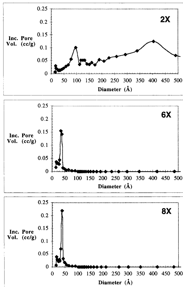
Figure 11. Incremental pore volume distribution plots of xerogels (2X, 6X, and 8X) prepared by base-catalyzed sol–gel polymerizations of the acyclic monomer 2, cyclic disilsesquioxane 6, and tricyclic dimer 8, respectively.
