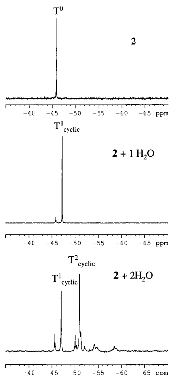
Figure 5. ^{29}\text{Si} NMR spectra for 1 M solutions of monomer 1,3-bis-(triethoxysilyl)propane 2 in ethanol. The top spectrum is that of the unreacted monomer. The next spectra are those of the product of the acid-catalyzed hydrolysis of each monomer with 1 (middle) and 2 (bottom) equiv of water. Spectra were obtained after 4 h; chromium acetoacetate (5 mmol/L) was added to each solution just before analysis. T^1_{\text{cyclic}} refers to the peak due to the cyclic disilsesquioxane 6 that formed from the intramolecular condensation of 2 . T^2_{\text{cyclic}} refers to the peak due to the tricyclic dimer 8 .
