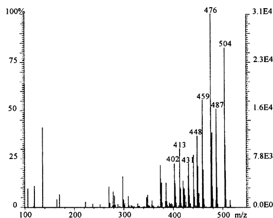
Figure 4. Mass spectrum (CI, \text{NH}_3 ) of the hydrolysis and condensation products of 1,2-bis(triethoxysilyl)ethane 1 with 1 equiv of water under acidic conditions. The products are predominantly the bicyclic dimer 4 and its hydrolysis products.
