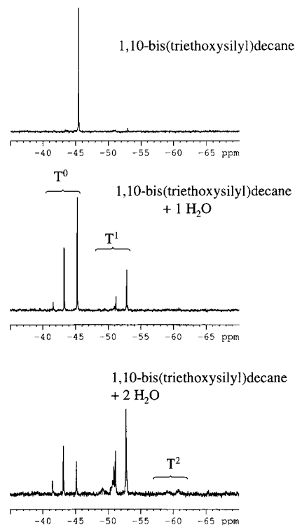
Figure 2. 29 Si NMR spectra for 1 M solutions of 1,10-bis(triethoxysilyl)decane in ethanol. The top spectrum is that of the unreacted monomer. The next spectrum is that of the product of the acid-catalyzed hydrolysis of the monomer with 1 (middle) and 2 (bottom) equiv of water. Spectra were obtained after 4 h; chromium acetyl acetonate (5 mmol/L) was added to each solution just before analysis. T 0 refers to the monomer and its hydrolysis products. T 1 refers to the peaks from silicons with a single siloxane bond (dimer or end-groups) and their hydrolysis products. T 2 refers to peaks from silicons with two siloxane bonds.
