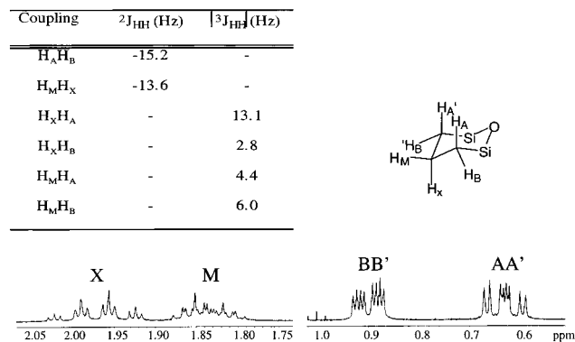
Figure 7. Expanded views of the ^1\text{H} resonances due to the \alpha and \beta hydrogens on the cyclic disilsesquioxane ring in 7 , revealing ^2J_{\text{HH}} and ^3J_{\text{HH}} couplings.
