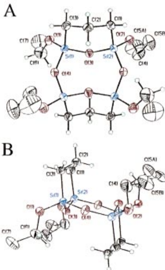
Figure 8. ORTEP plots of the X-ray crystal structure of the tricyclic dimer 8 , showing the anti configuration of the six-membered cyclic disilsesquioxane rings about the central eight-membered tetrasiloxane ring. The methyl carbon {C(5)} in 8 was modeled at two positions with a site occupancy factor of 0.72(4) for C(5A) and 0.28 for C(5B). This was done because the anisotropic thermal ellipsoid was too large to be appropriate for one site. Packing within the structure suggests that the ends of the ethyl groups are free to move in an interpenetrating fashion between the planes of the molecules, which would allow them to rotate due to thermal motion, giving rise to the disorder.
