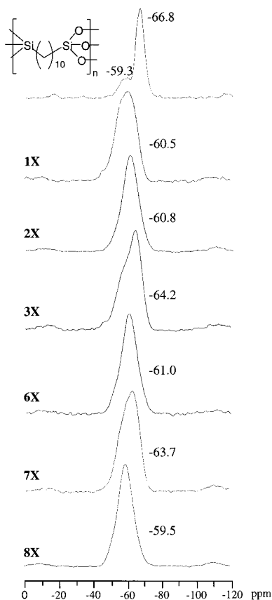
Figure 10. Comparison of the solid-state ^{29}\text{Si} CP MAS NMR spectrum of a decylene-bridged polysilsesquioxane (top) with spectra of xerogels ( 1X–3X ) obtained from monomers 1–3 that are capable of forming cyclics and with spectra of xerogels ( 6X–8X ) prepared from cyclic monomers 6–8 .
