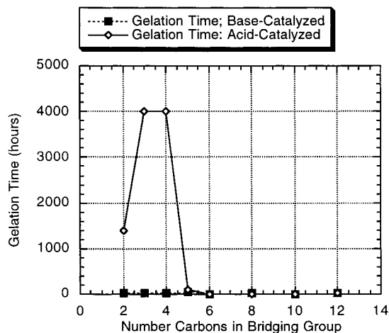
Figure 1. Gelation times for \alpha,\omega -bis(triethoxysilyl)alkanes (0.4 M in ethanol, 6 H 2 O), 10.8 mol % HCl or NaOH catalyst).
