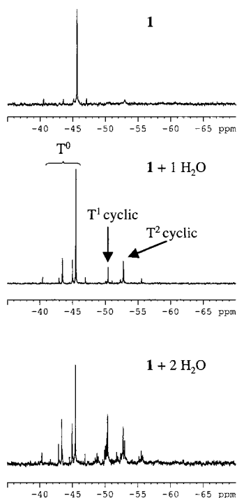
Figure 3. ^{29}\text{Si} NMR spectra for 1 M solutions of monomer 1 in ethanol. The top spectrum in each series is that of the unreacted monomer. The next spectra are those of the product of the acid-catalyzed hydrolysis of each monomer with 1 (middle) and 2 (bottom) equiv of water. Spectra were obtained after 4 h; chromium acetyl acetonate (5 mmol/L) was added to each solution just before analysis. T^0 refers to the monomer and its hydrolysis products. T^1_{\text{cyclic}} and T^2_{\text{cyclic}} refer to the peaks due to silicons with a single siloxane bond and two siloxane bonds, respectively, that are part of a seven-membered disilsesquioxane ring, such as in compound 5 .
